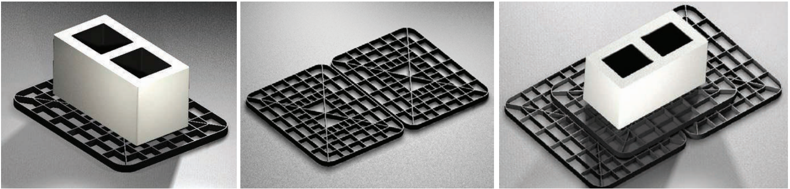
STEP 1 - 17" x 22" ABS Pad STEP 2 - (2) 17" x 22" ABS PADS (34" x 22" Configuration) STEP 3 - Complete Assembly 34" x 22" Multi-pad Configuration
