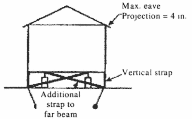
Second Beam Method (Vertical tie down straps required)
