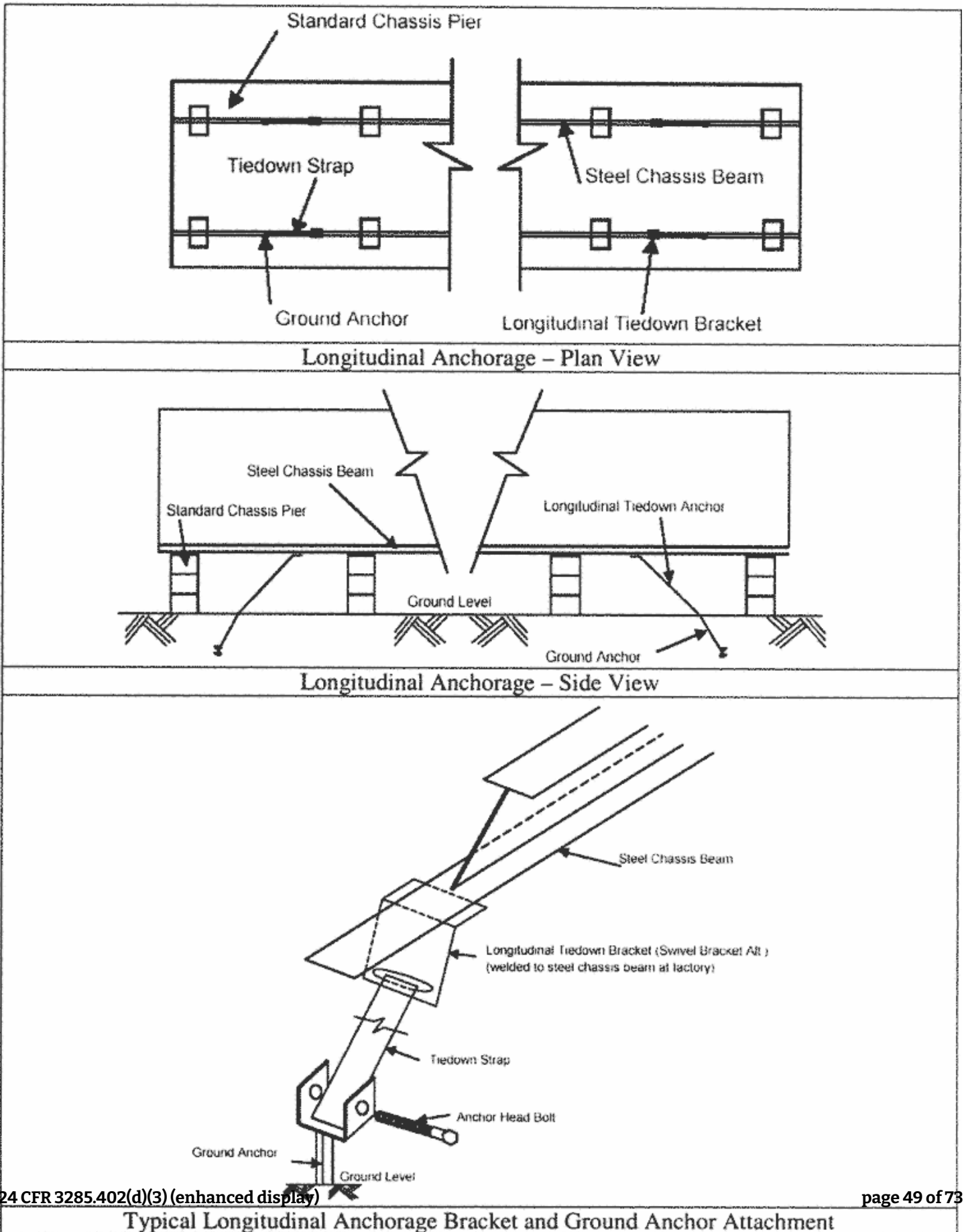
Figure C to § 3285.402 Longitudinal Anchoring
