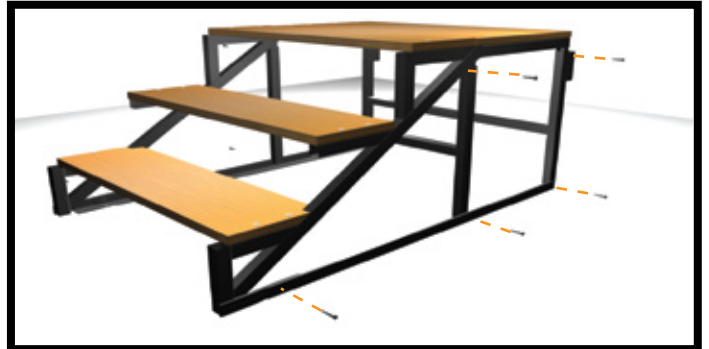
6. Secure with 3/4 inch tech screws. (5 per side)
